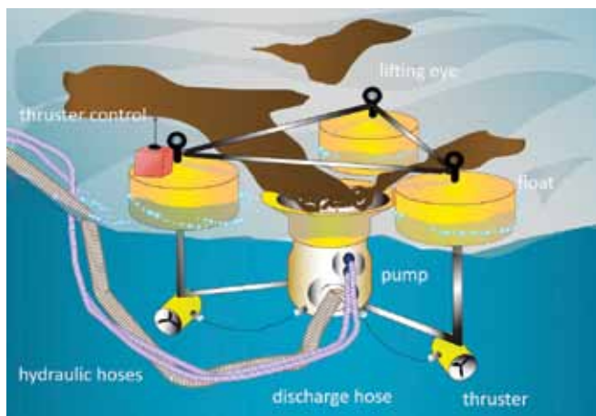
▲ Figures 12 and 13: A weir skimmer selectively recovers oil over the top of the central weir sited just below the upper surface of the slick by the force of gravity into a central reservoir where it is pumped to storage.
